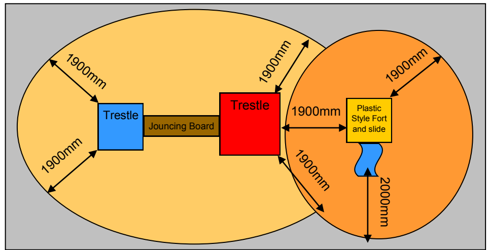
Figure 1 —Minimum dimensions of fall zones for mobile equipment in supervised early childhood settings ( Kidsafe NSW recommendation).
